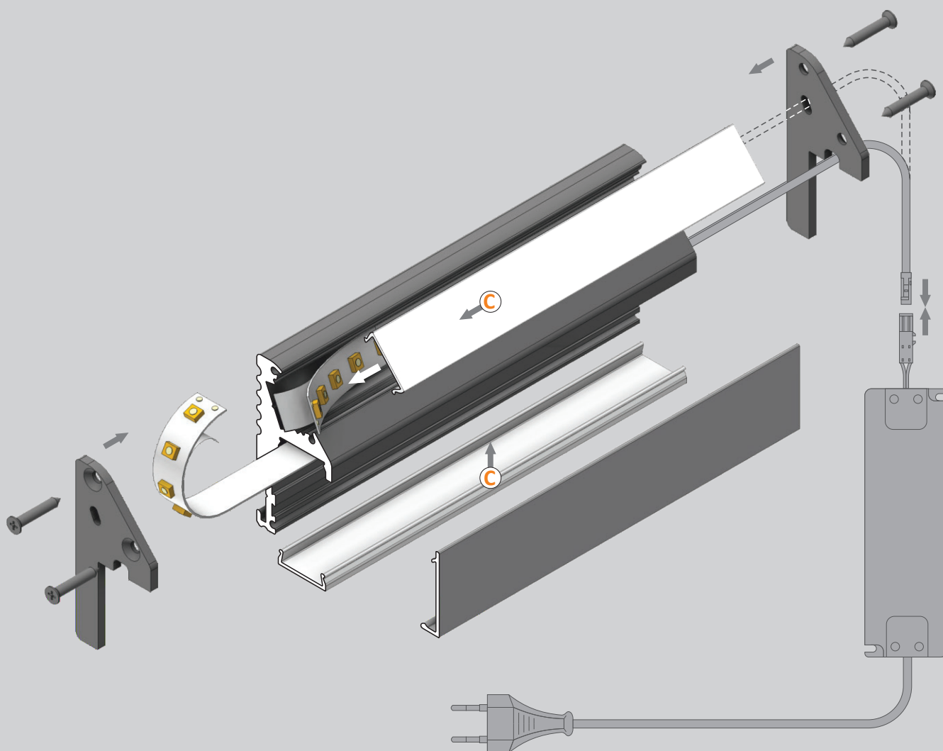
mounting options
