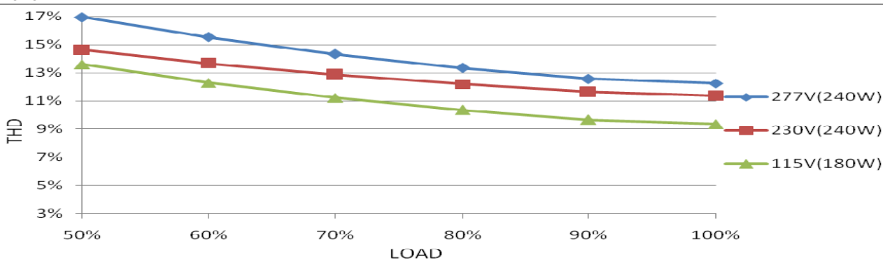
THD vs LOAD
