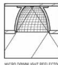
MICRO DOWNLIGHT REFLECTOR
