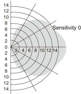
Wall Pattern (Unit: m) Installation Height: 10m
