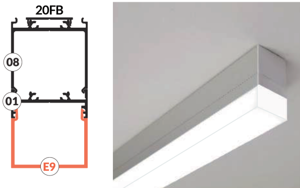
variant 15 - ceiling 20FB-08-01-E9 wariant 15 - sufitowy 20FB-08-01-E9
