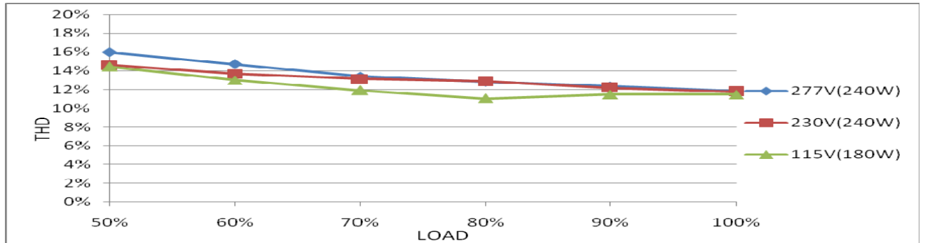
THD vs LOAD
