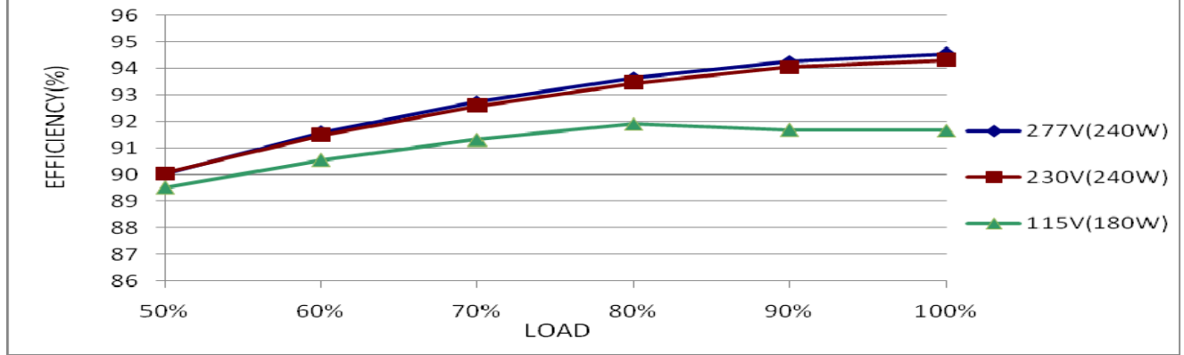
EFFICIENCY vs LOAD
