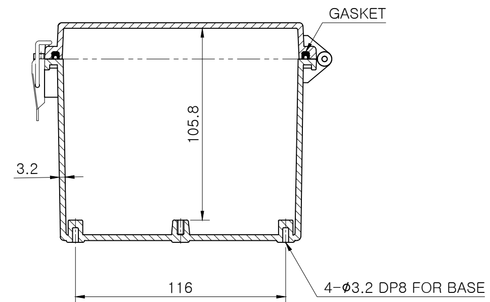
SECTION B-B
