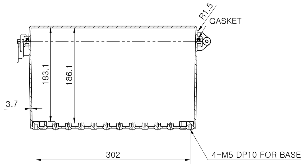
SECTION B-B
