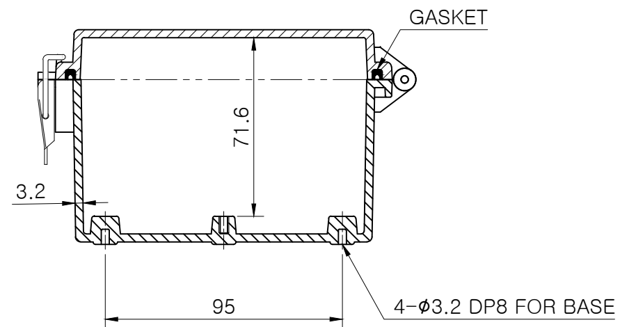
SECTION B-B
