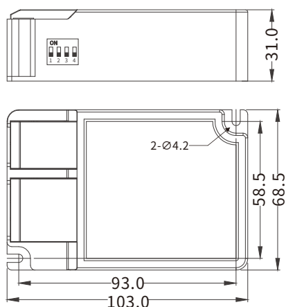
DUL030-B/DUL042-B
